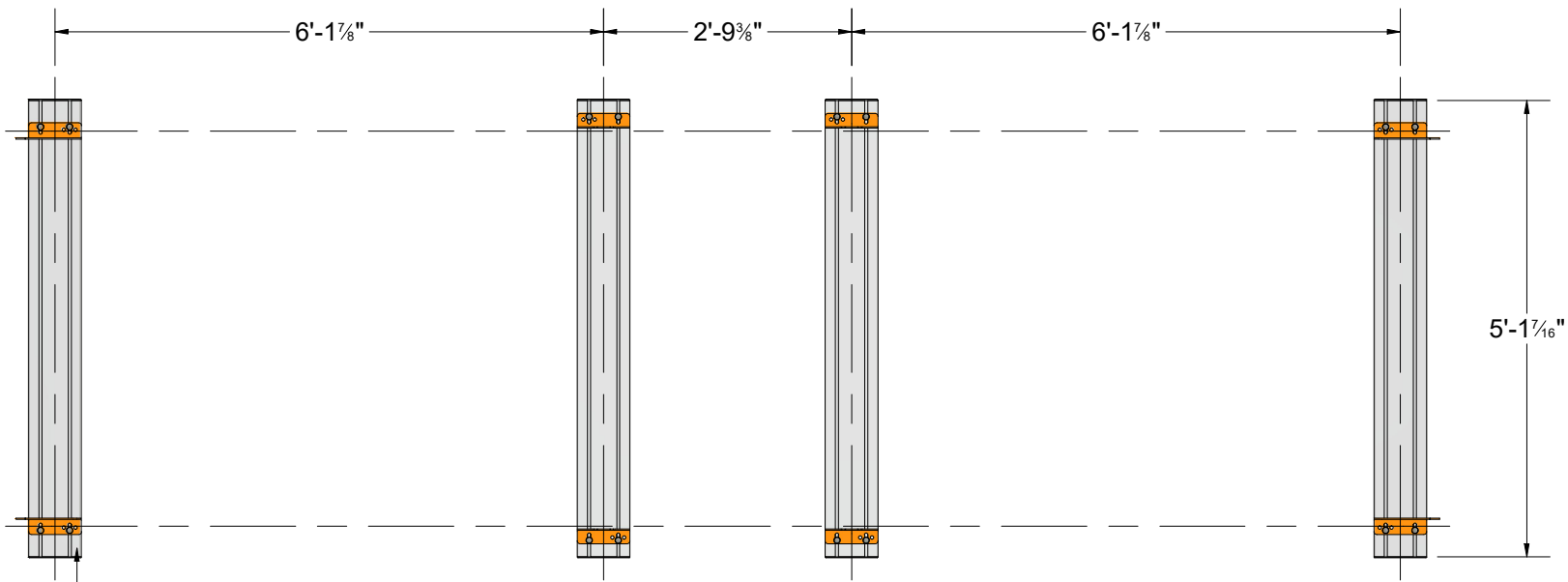
FOOTING LAYOUT
