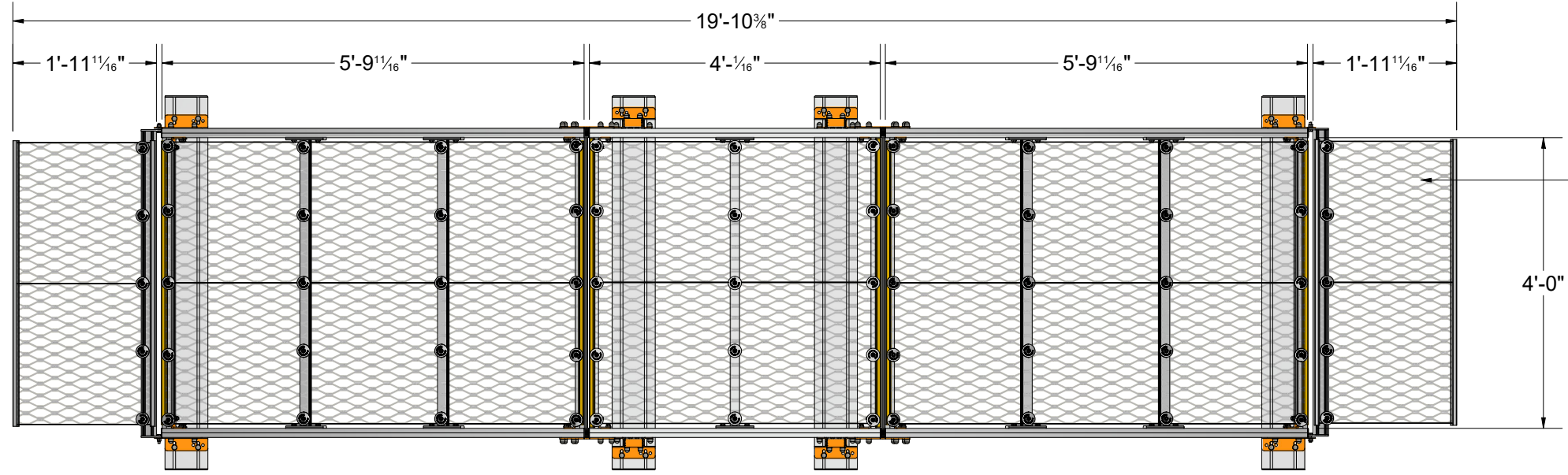
TOP VIEW
